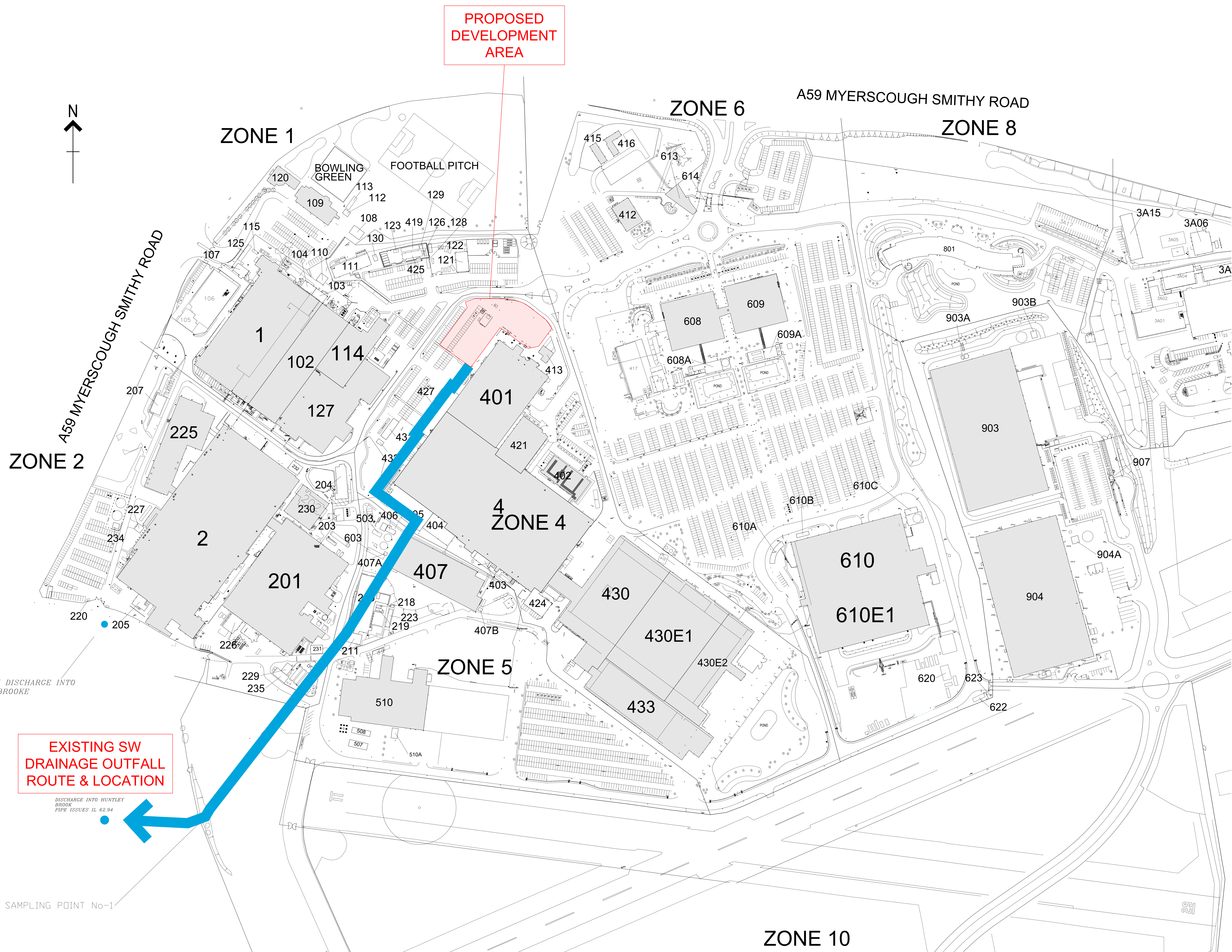
EXISTING SITE PLAN WITH SW DRAINAGE OUTFALL ROUTE & LOCATION
