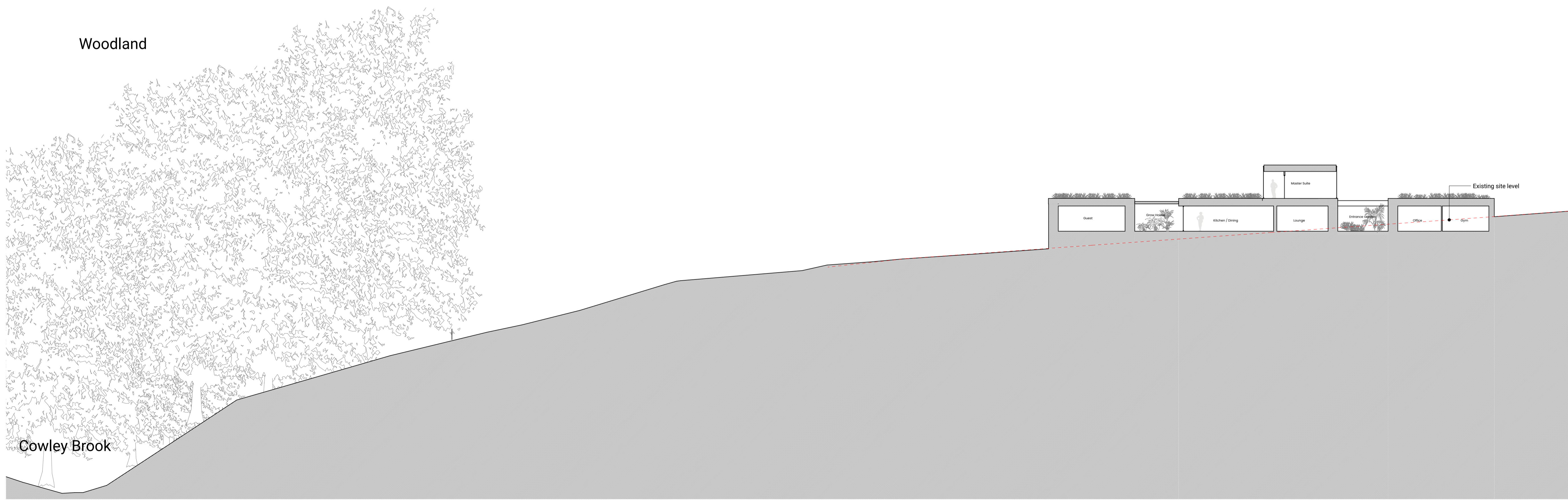
Section C-C 1:200
