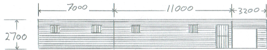
PROPOSED FRONT ELEVATION (NORTH)
