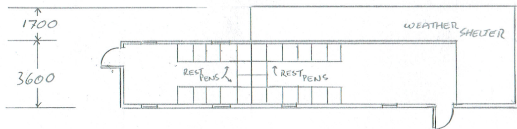
PROPOSED FLOOR PLAN
