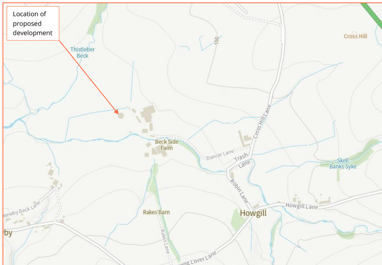
Figure 10: Extract from Environment Agency Reservoir Flood Map (Source: EA)
