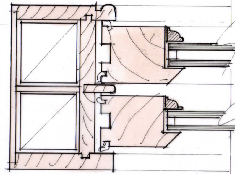
BOX SASH WITH WEIGHTS - HORIZONTAL SECTION SCALE 1:2 @ A3
