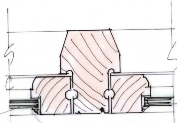
HORIZONTAL SECTION WITH MULLION
