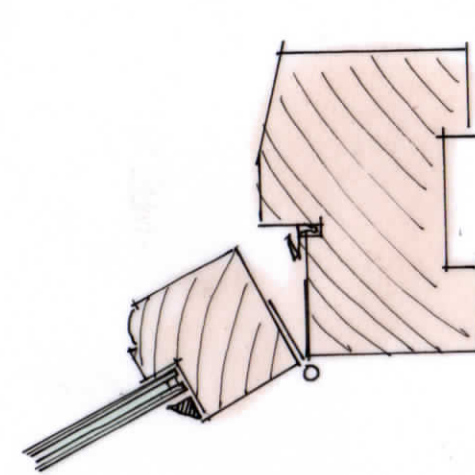
HORIZONTAL SECTION - FRAME
