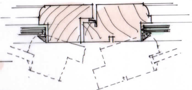
HORIZONTAL SECTION WITH STILE OPENING
