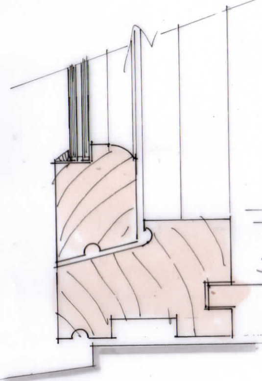
HORIZONTAL SECTION WITH MULLION
