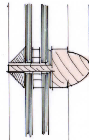
GLAZING BAR SCALE 1:1 @ A3
