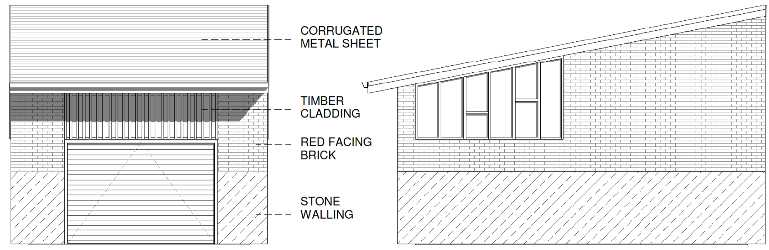
2 Front Elevation 1:50
