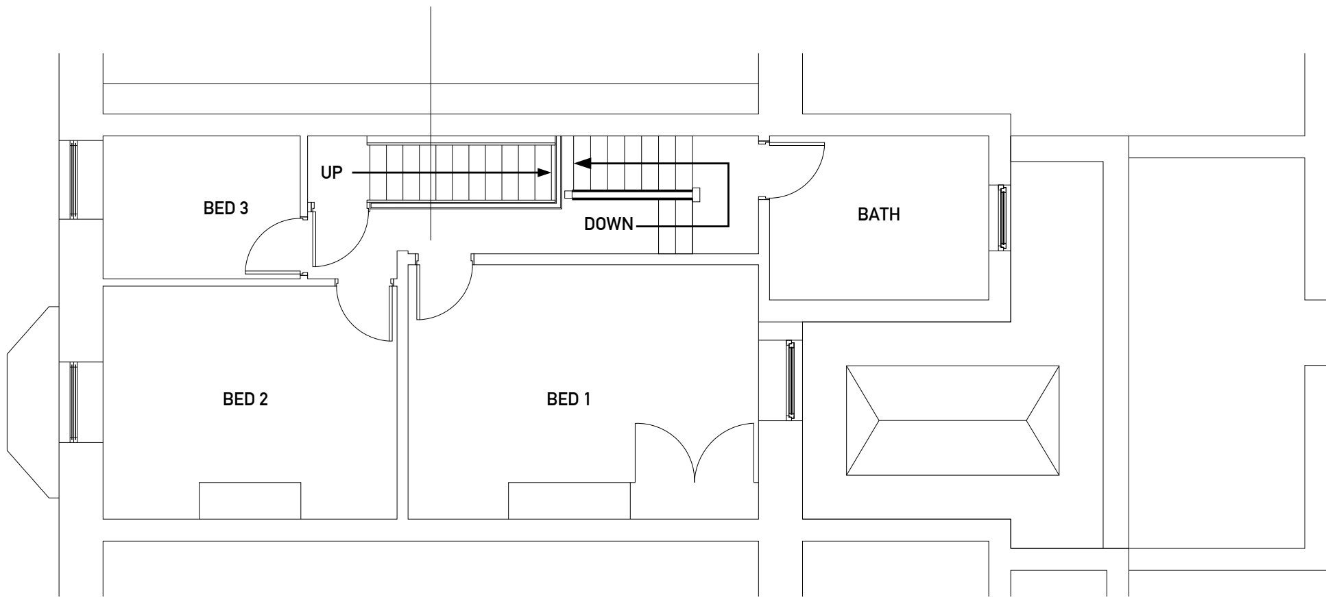
PROPOSED 1ST FLOOR PLAN OPT 2
