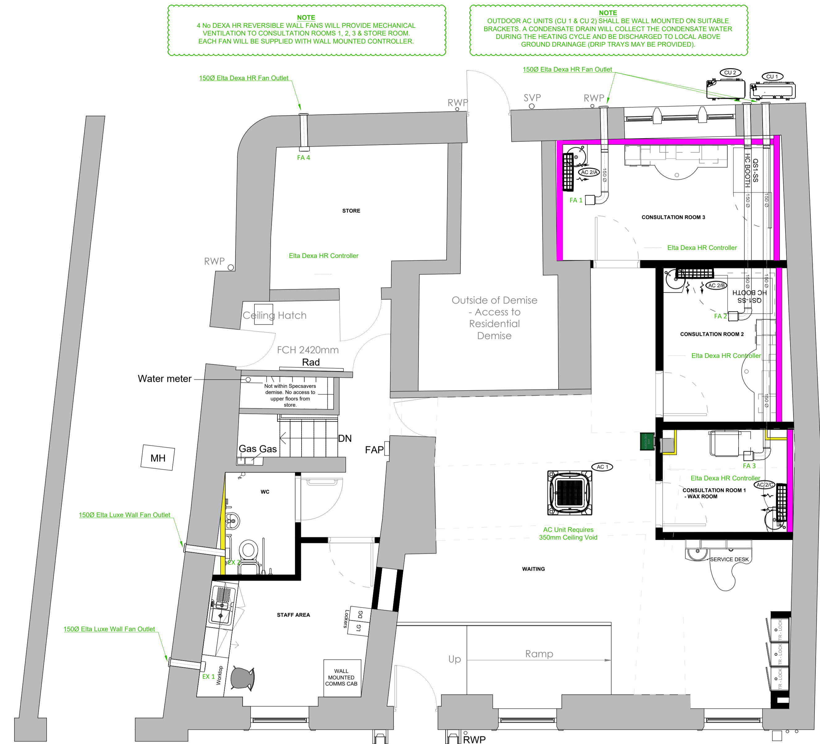
PROPOSED LAYOUT SCALE 1:50 @A1
