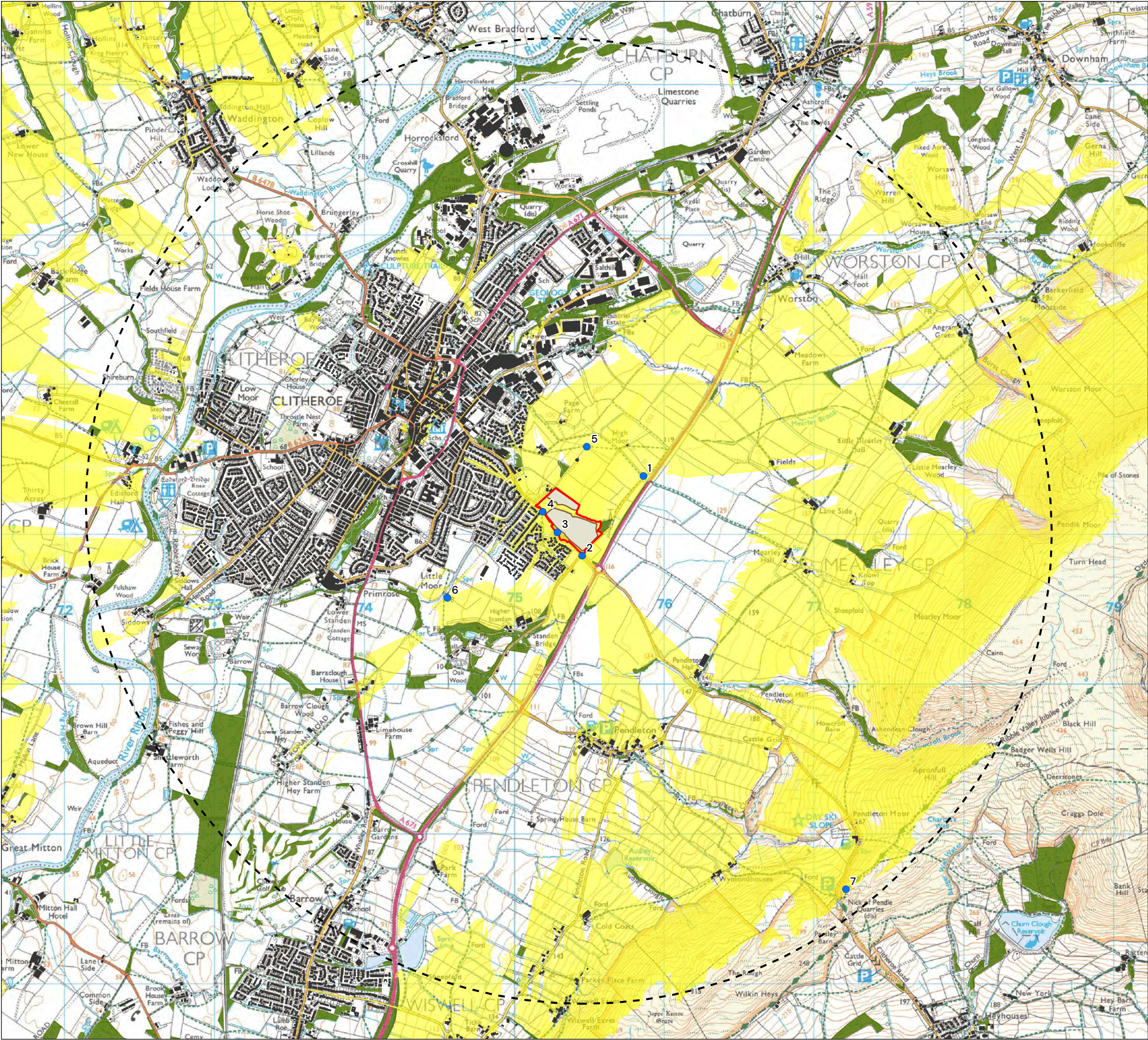
FIGURE 4: SCREENED ZONE OF THEORETICAL VISIBILITY WITH VIEWPOINT LOCATIONS
