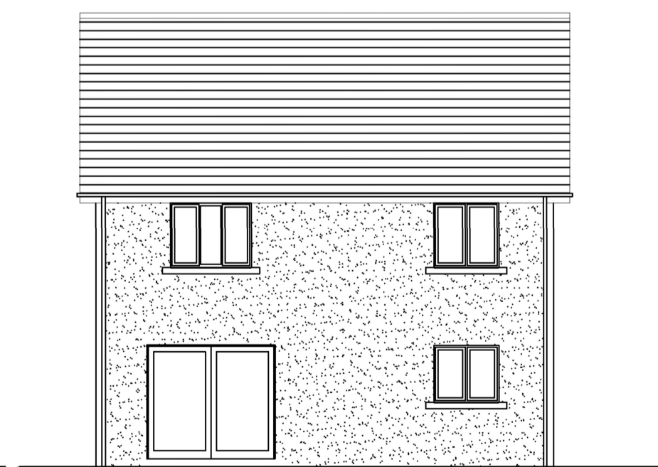
REAR ELEVATION
