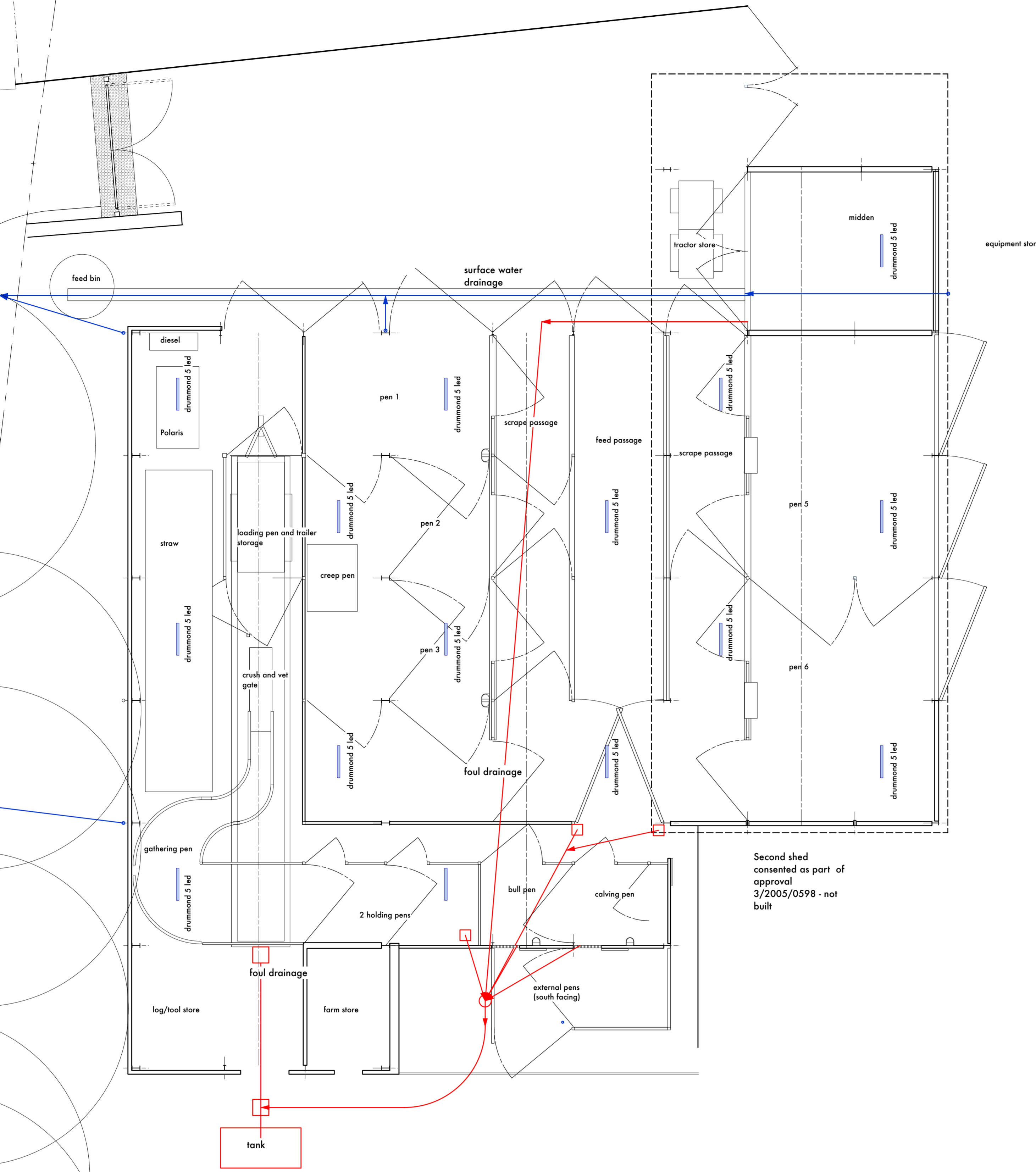
B Proposed Floor Plan 1:100
