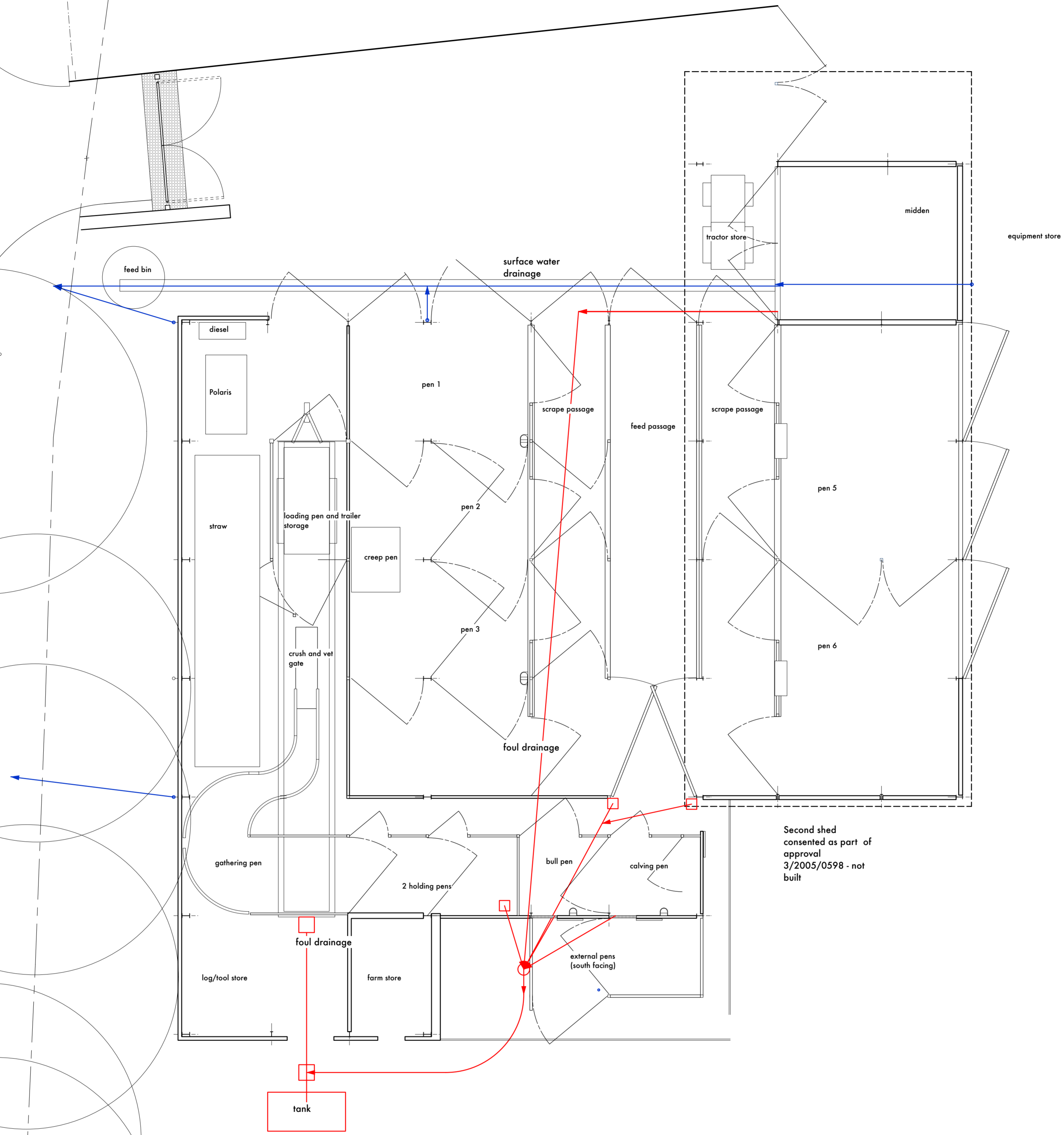
B Proposed Floor Plan 1:100
