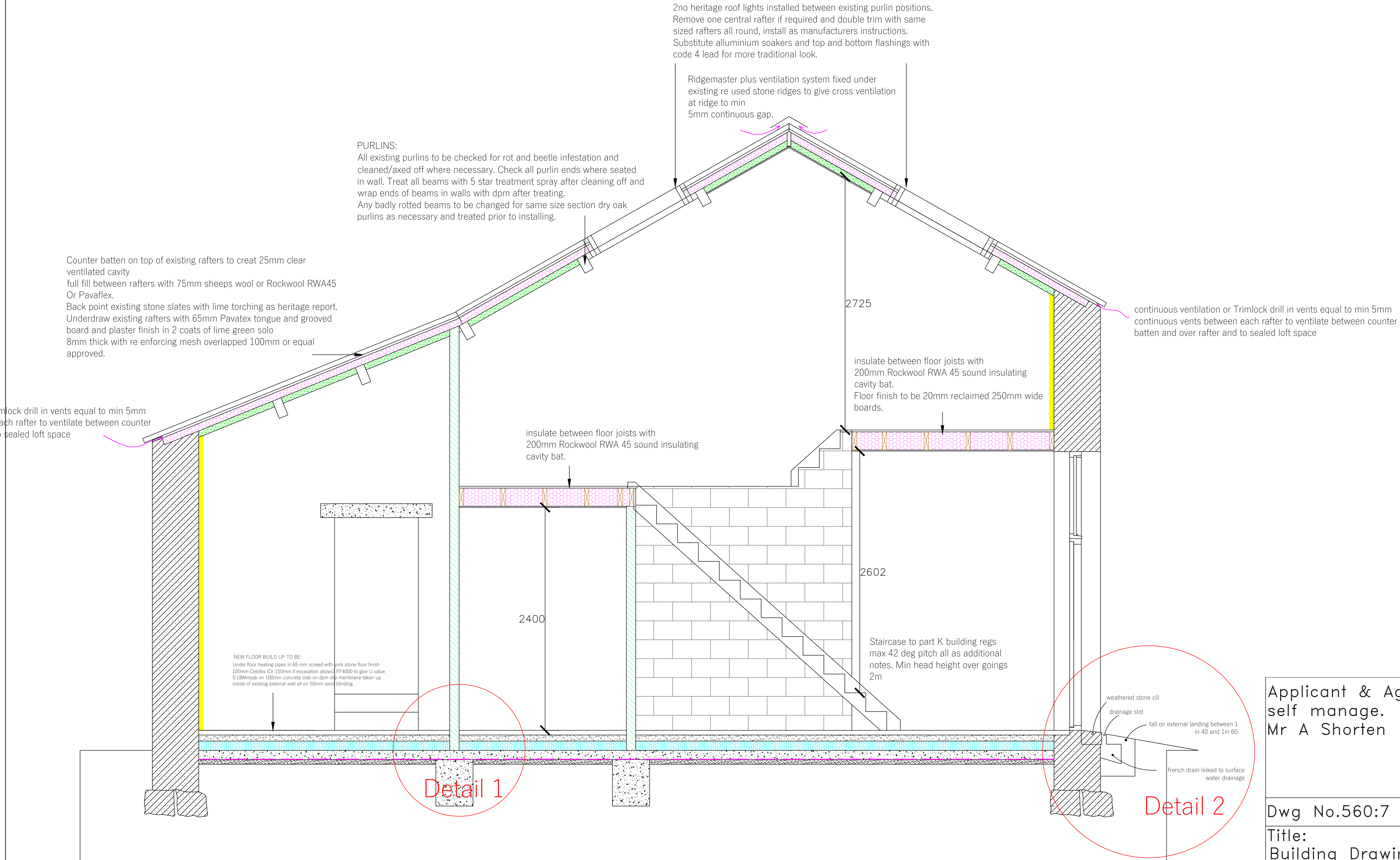
SECTION C-C
