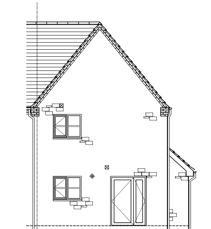
REAR ELEVATION
