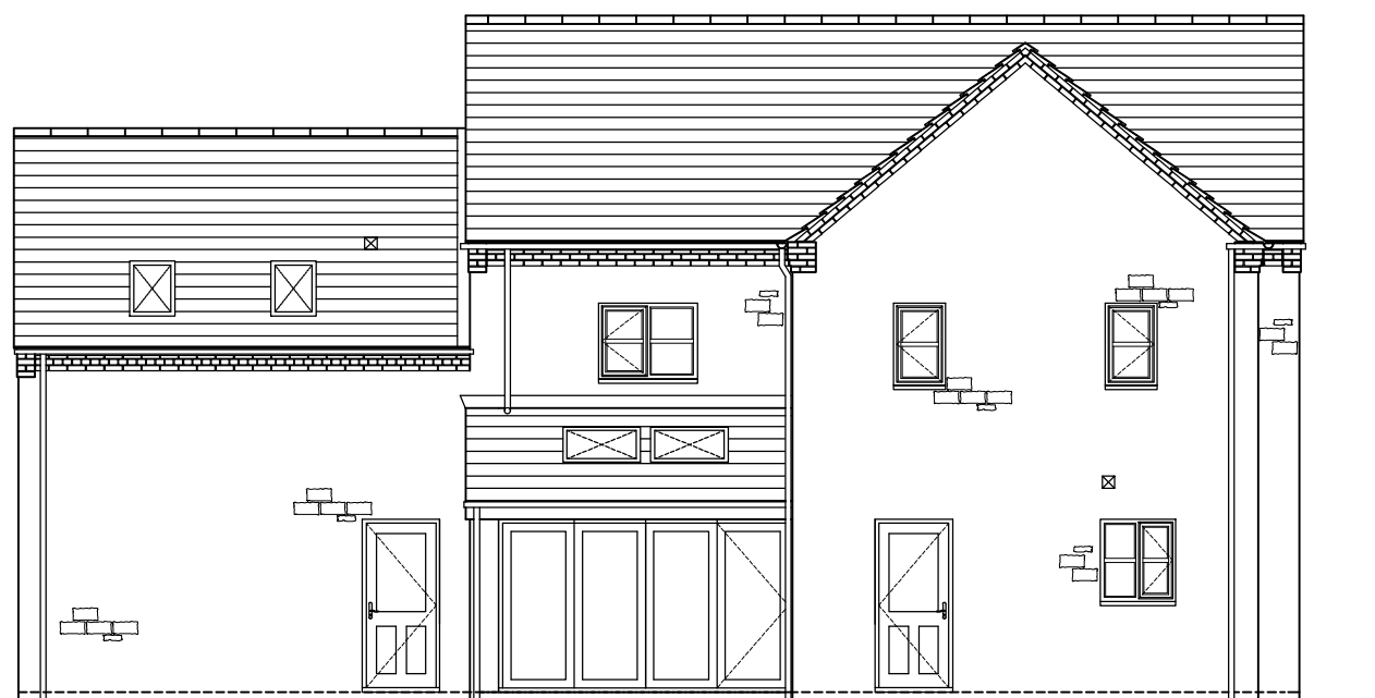
REAR ELEVATION
