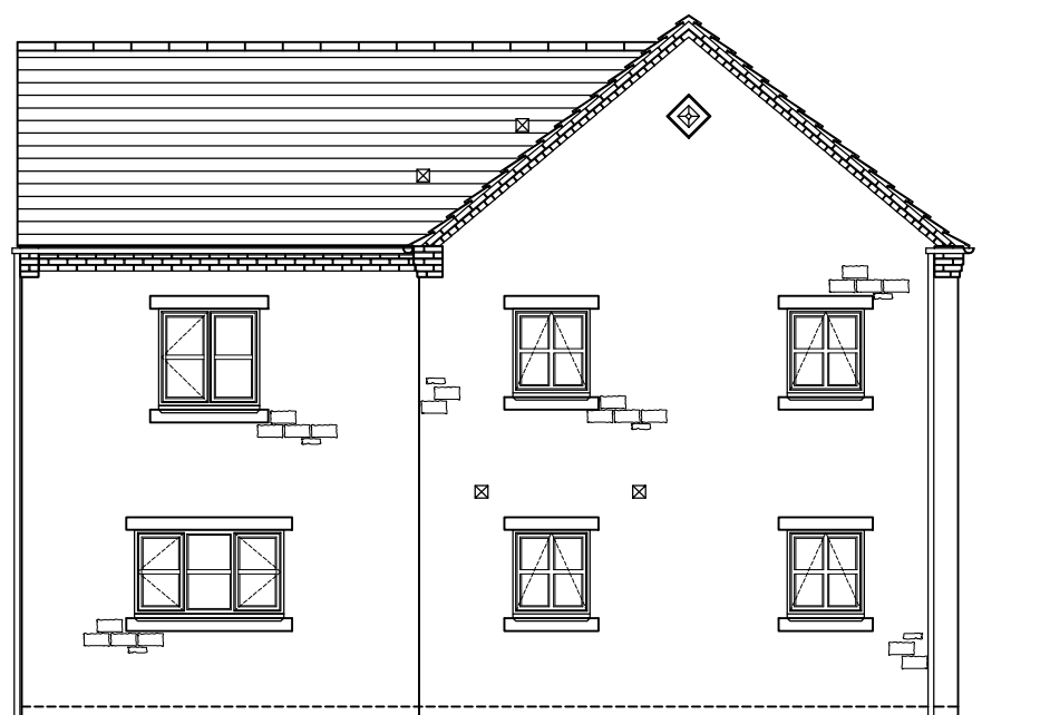
EXPOSED SIDE ELEVATION
