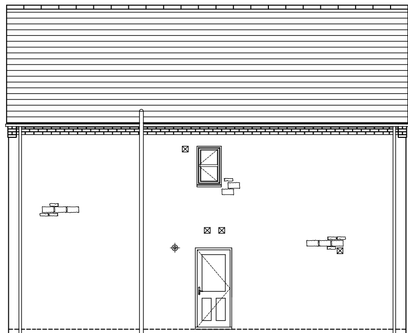
REAR ELEVATION
