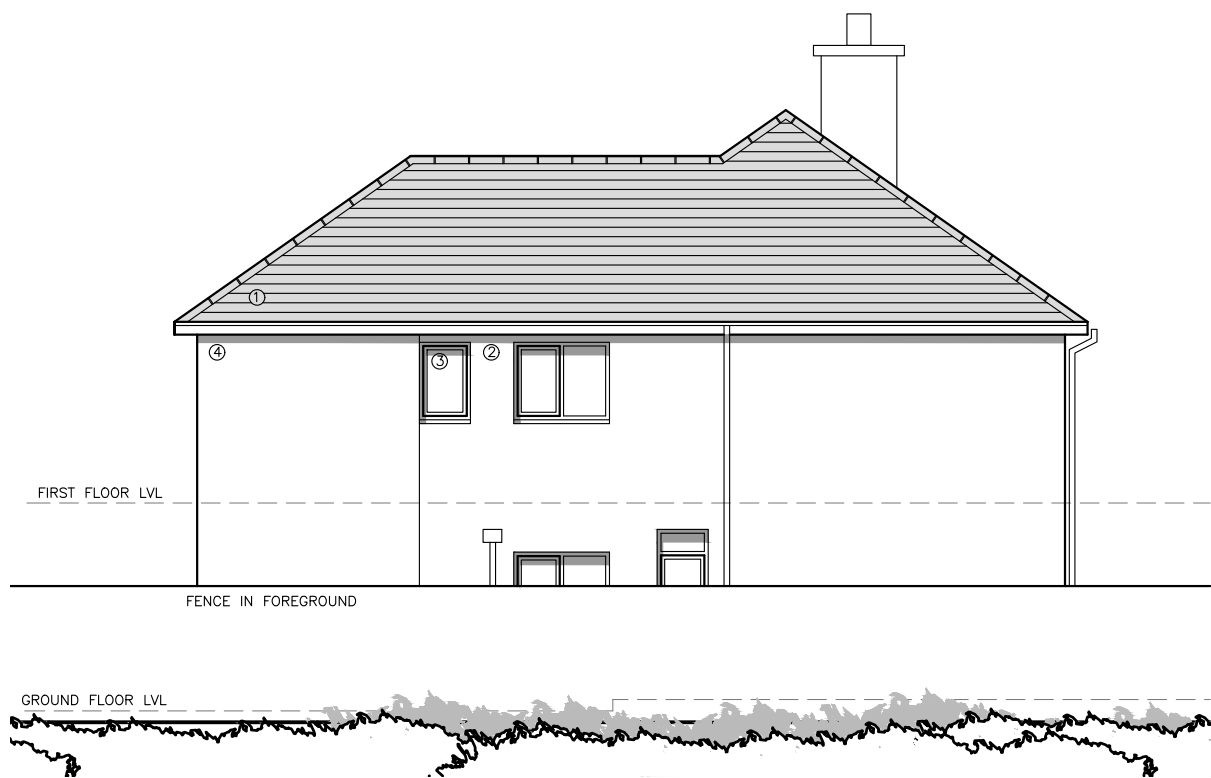
PROPOSED SIDE ELEVATION (3)
