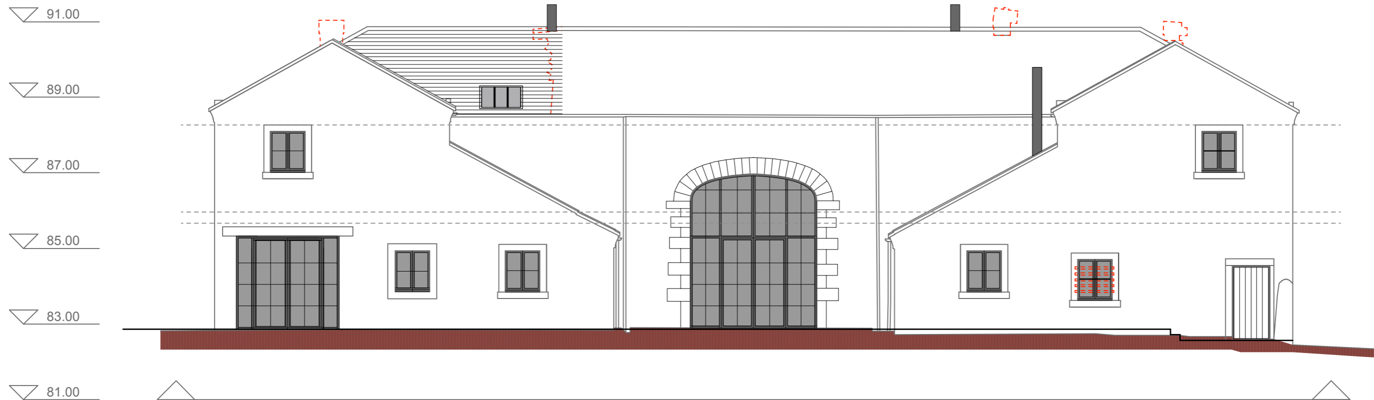
FRONT ELEVATION
