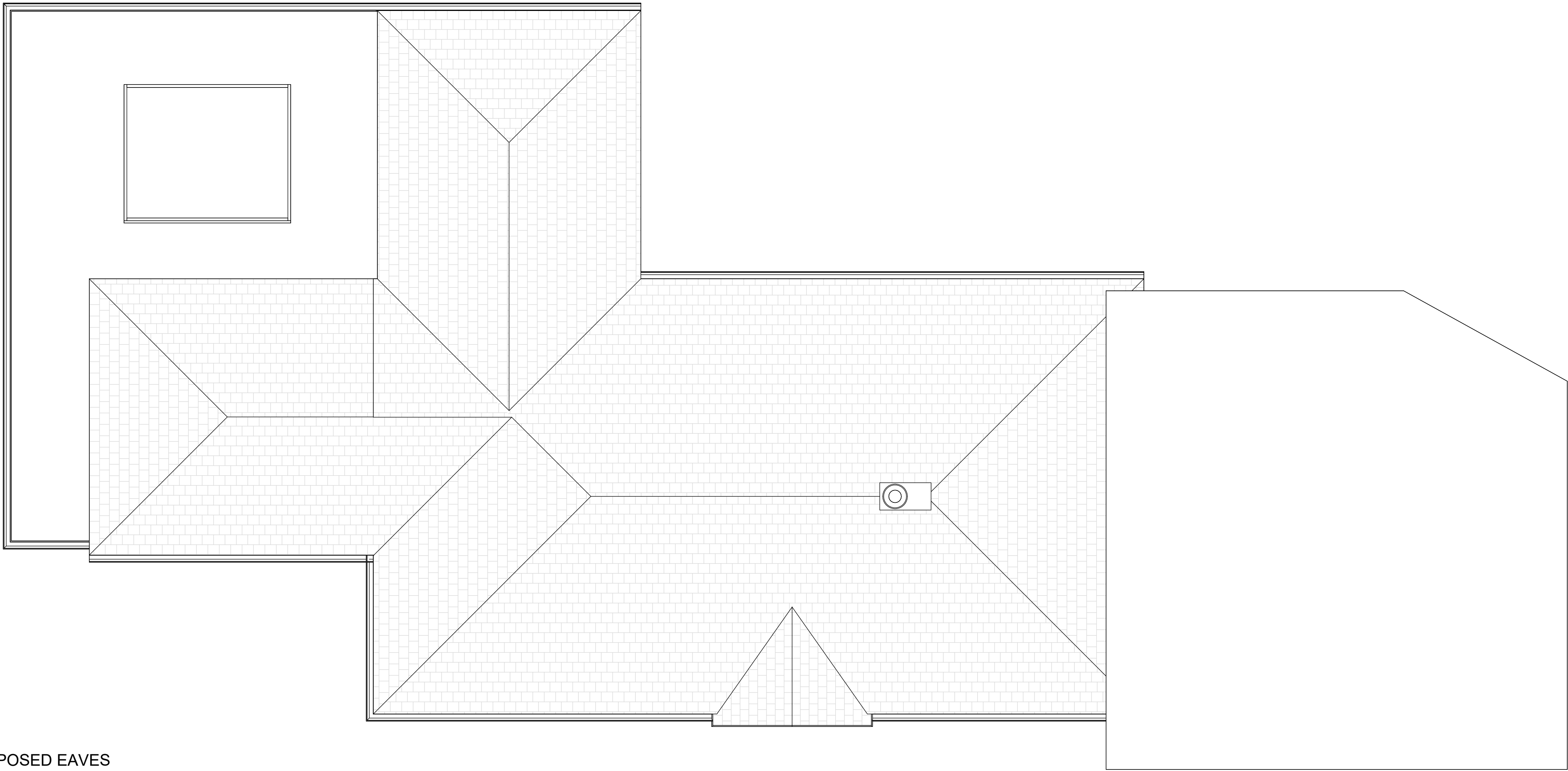
2 PROPOSED EAVES 1 : 50
