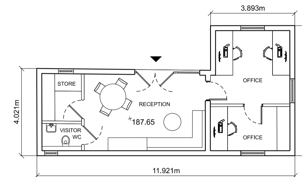
Proposed Office / Reception Plan Scale 1:100
