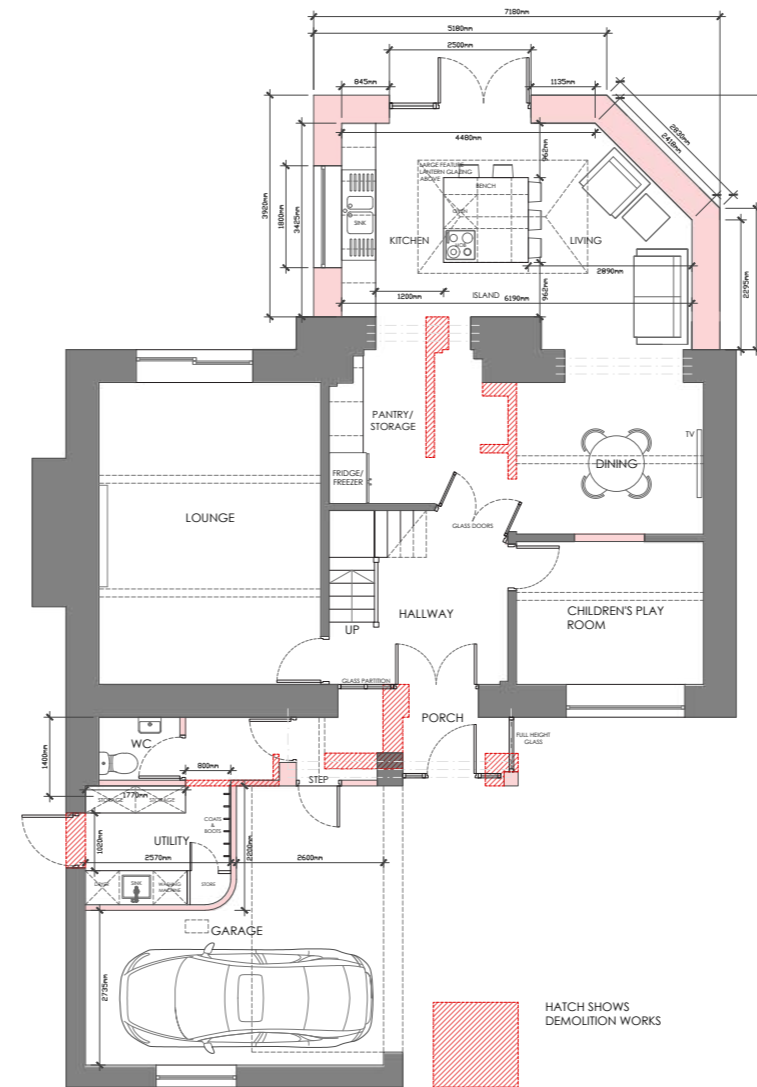
PROPOSED GROUND FLOOR PLAN Scale 1:50
