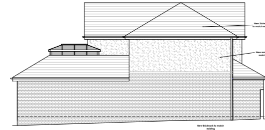
PROPOSED SIDE ELEVATION Scale 1:100
