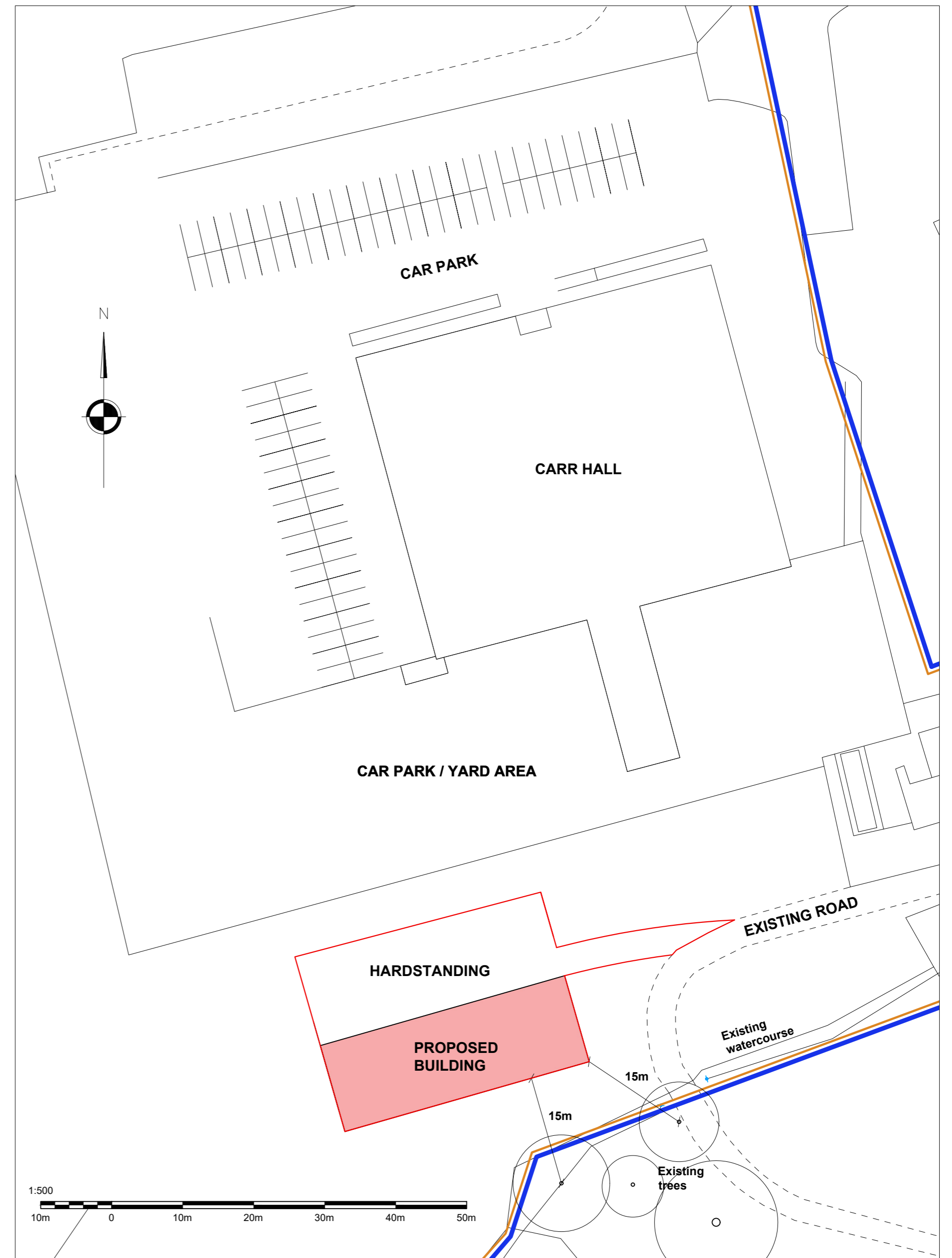
SITE LAYOUT AS PROPOSED Scale 1.500 @ A2
