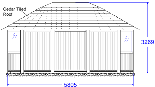
Back Elevation View
