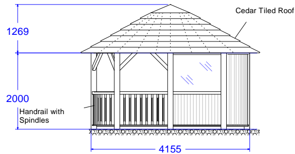
Side Elevation View Right
