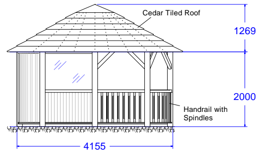
Side Elevation View Left
