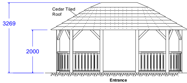
Front Elevation View
