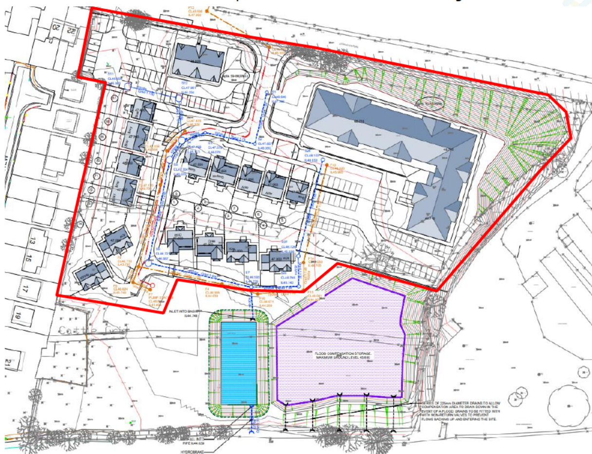
Figure 1-2: Proposed site plan (Phase 1)
