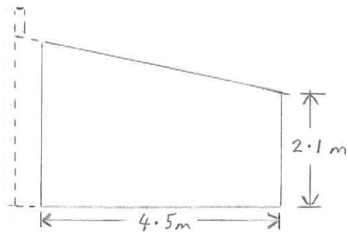
West Elevation
