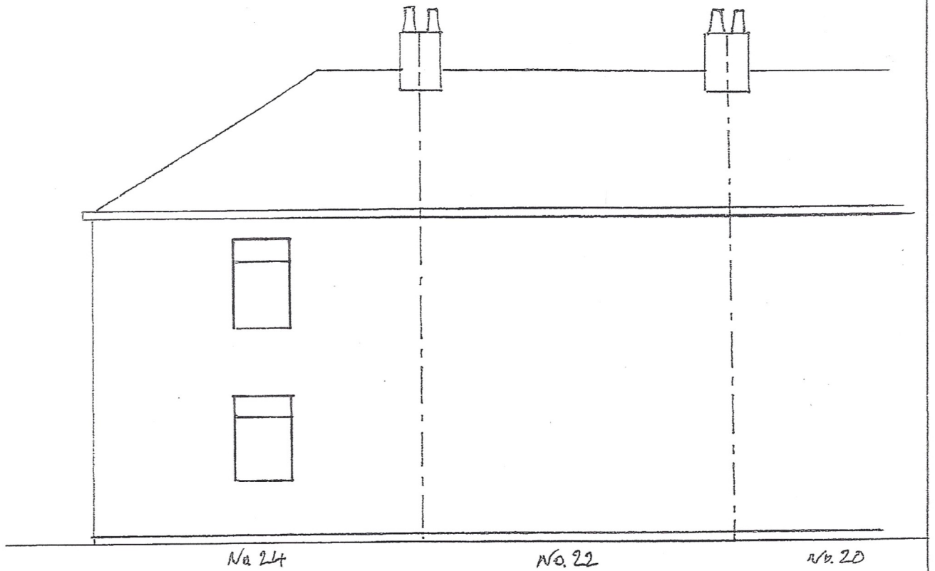
FRONT ELEVATION
