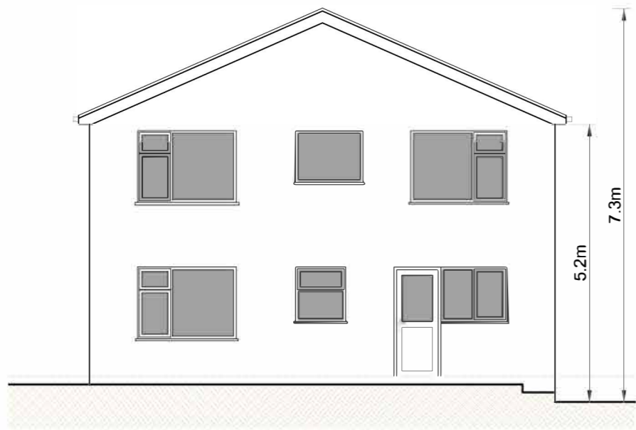
REAR ELEVATION
