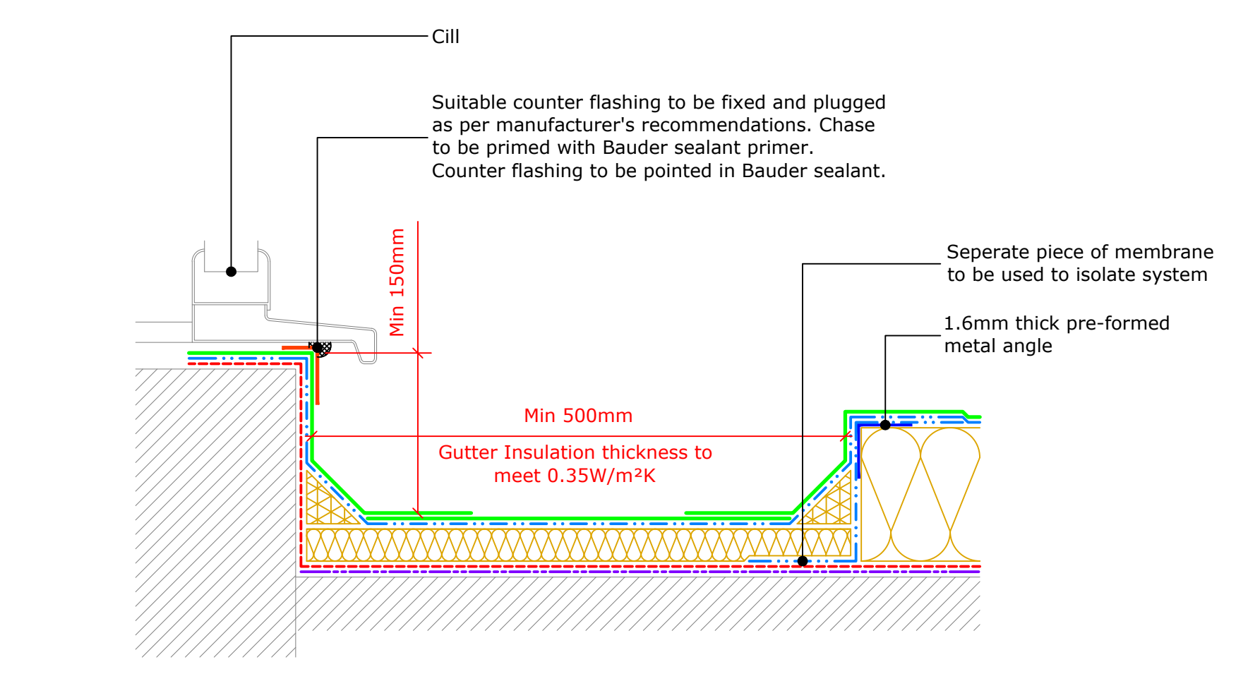
Internal Gutter to Clerestory Window (Drg.No: D0000-00W_006-004)
