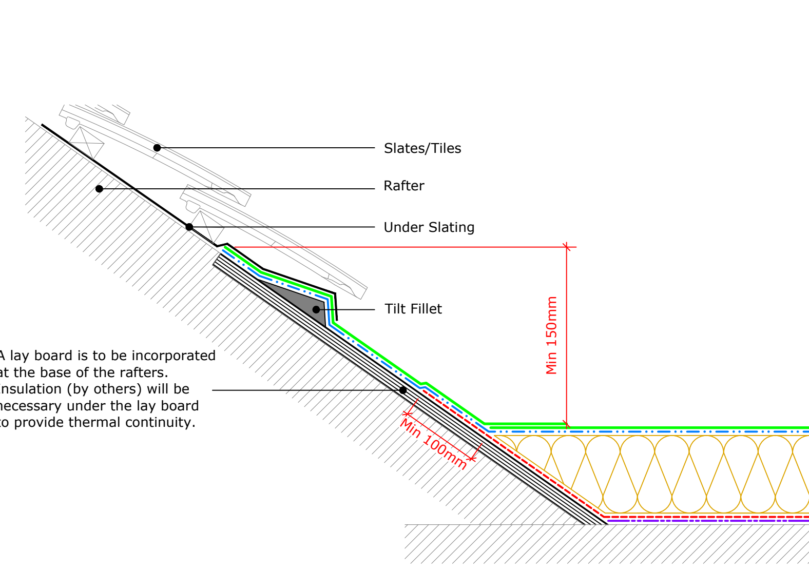
Upstand to Pitched Roof (Drg.No: D0000-00W_001-004)
