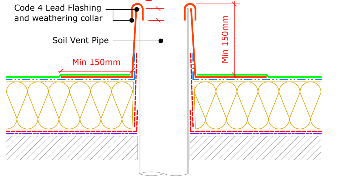
Soil Vent Pipe (Drg.No: D0000-00W_007-001)
