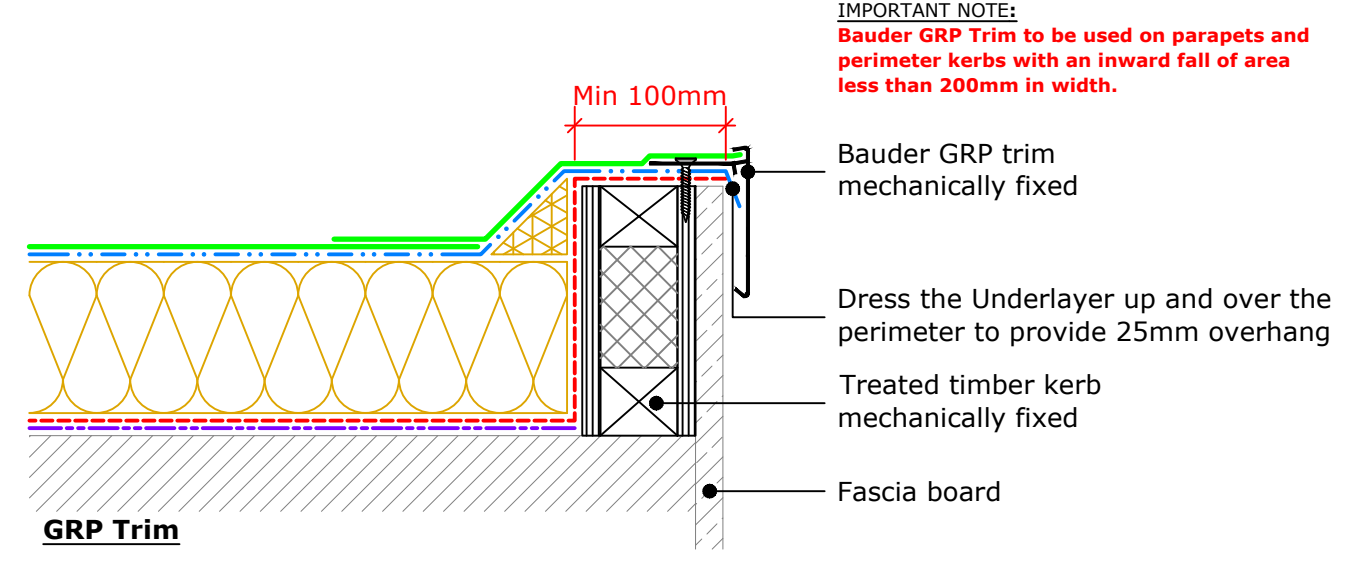
Perimeter Kerb (Drg.No: D0000-00W_002-001)
