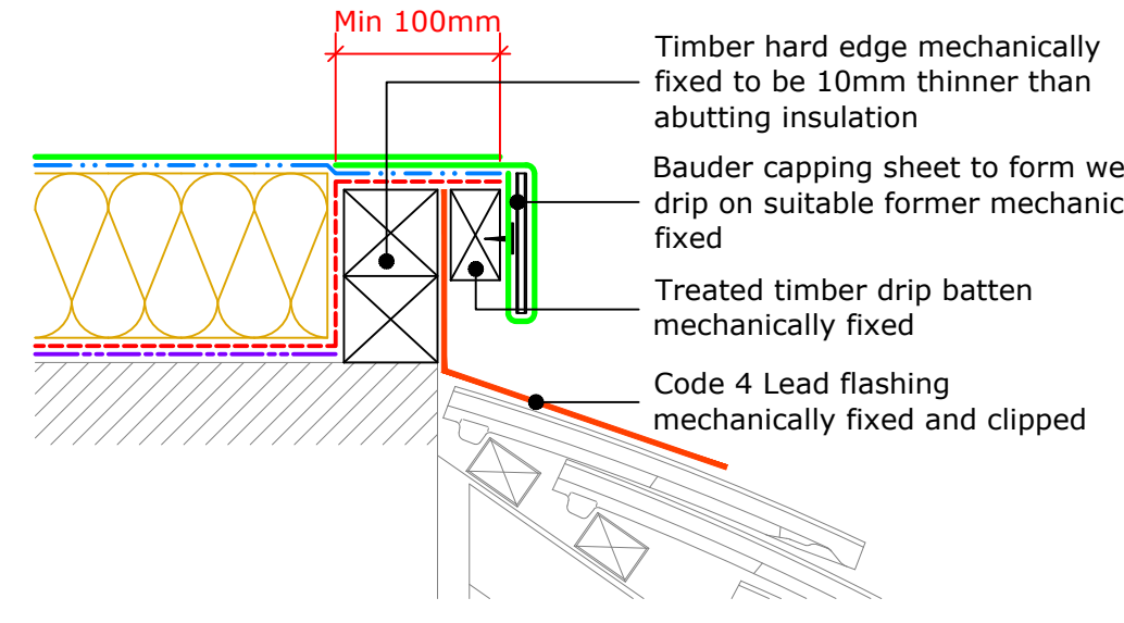
Detail to Mansard Roof (Drg.No: D0000-00W_006-006)
