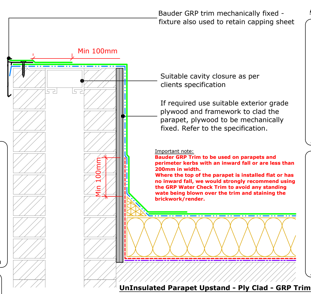
UnInsulated Upstand to Parapet (Drg.No: D0000-00W_103-001)
