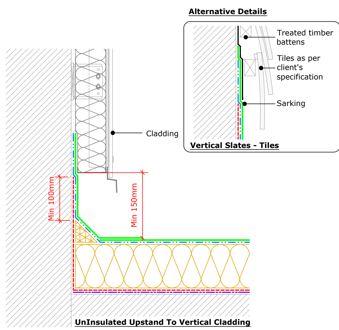
UnInsulated Upstand to New Vertical Cladding or Slates/Tiles (Drg.No: D0000-00W_101-002)
