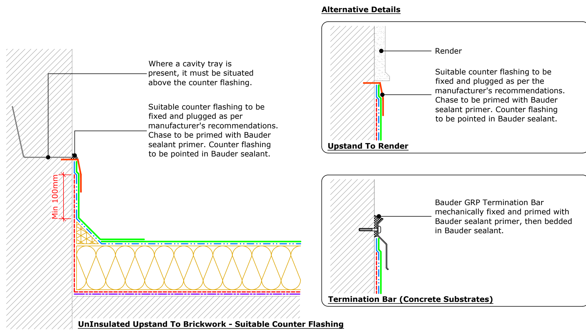
UnInsulated Upstand (Drg.No: D0000-00W_101-001)
