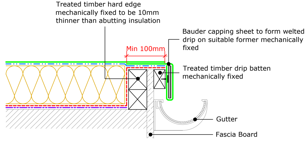
External Gutter (Drg.No: D0000-00W_005-005)
