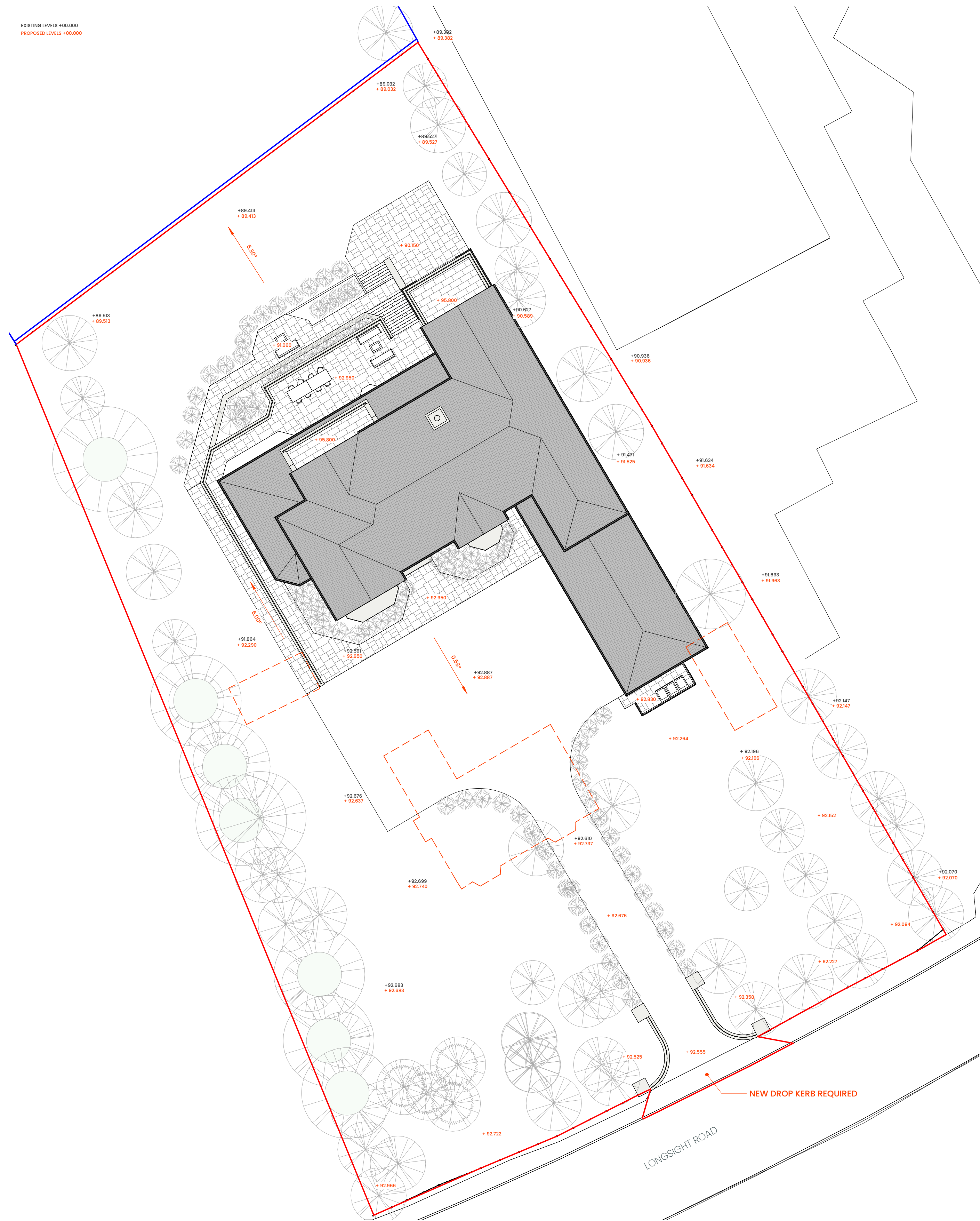
2 PROPOSED LEVEL PLAN - PLANNING 1:200
