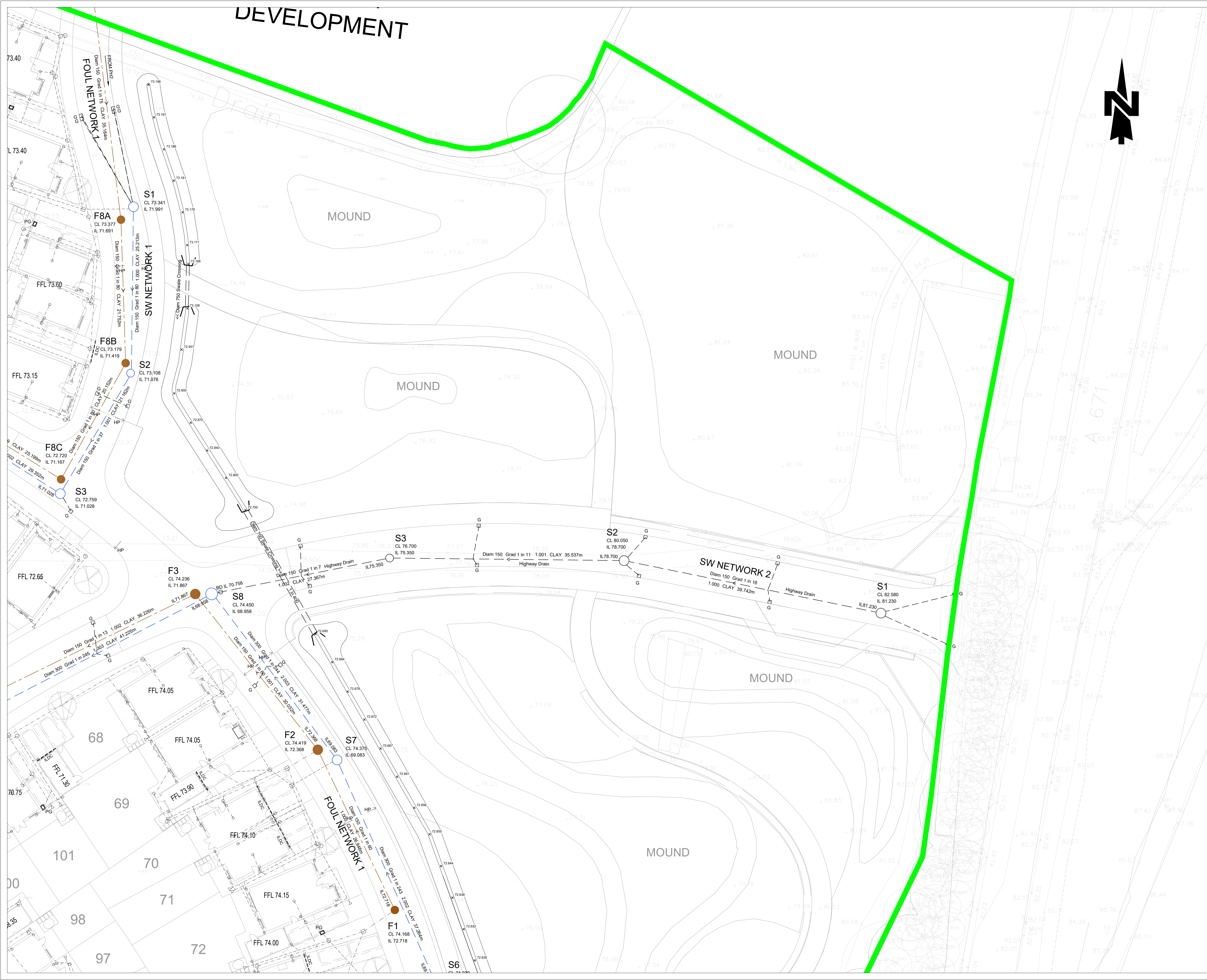
LOCATION PLAN 1:5000
