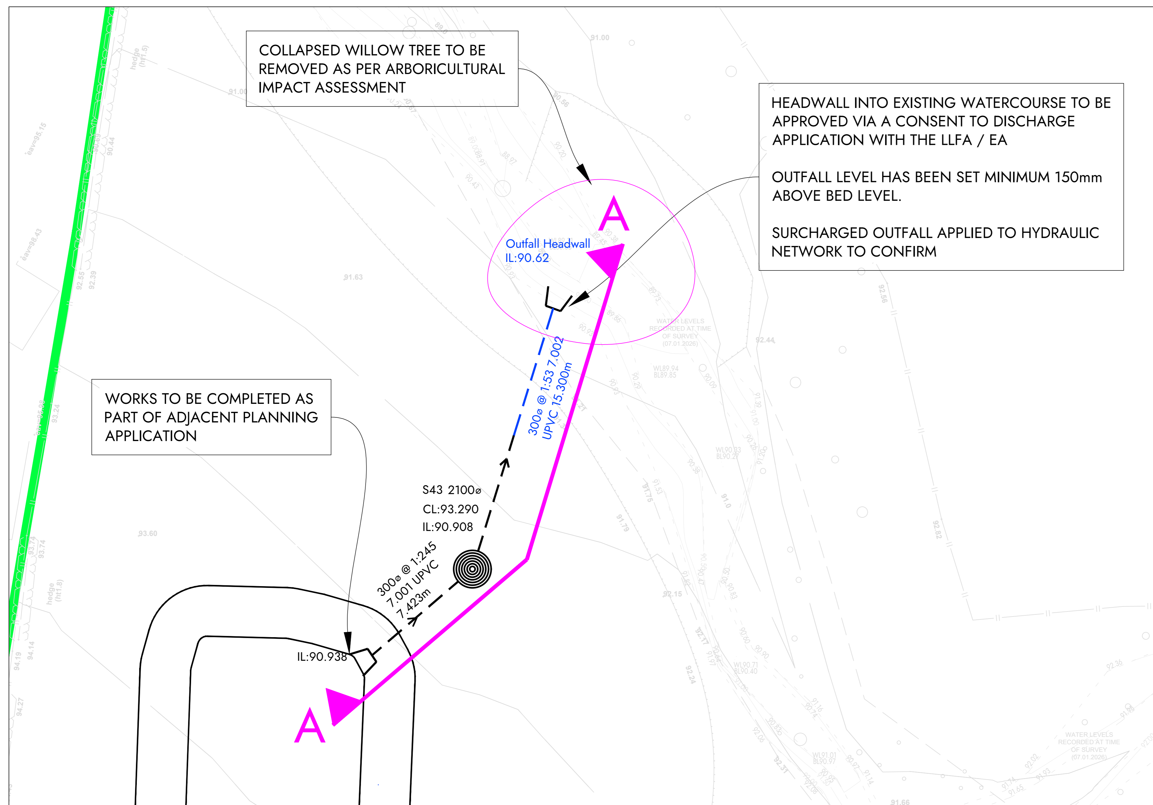
OUTFALL LOCATION PLAN @ 1:200
