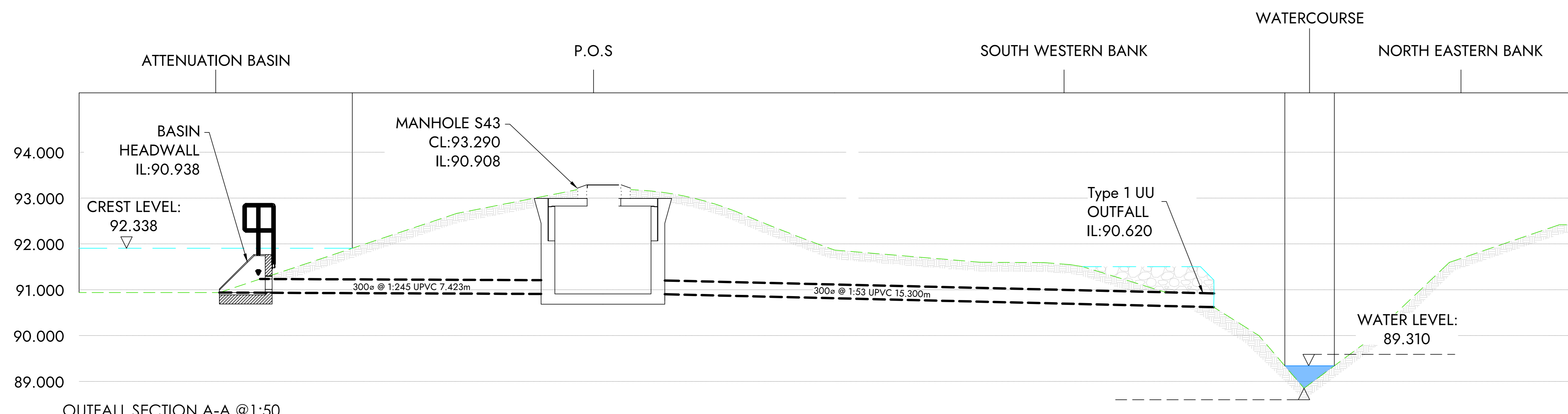
OUTFALL SECTION A-A @ 1:50
