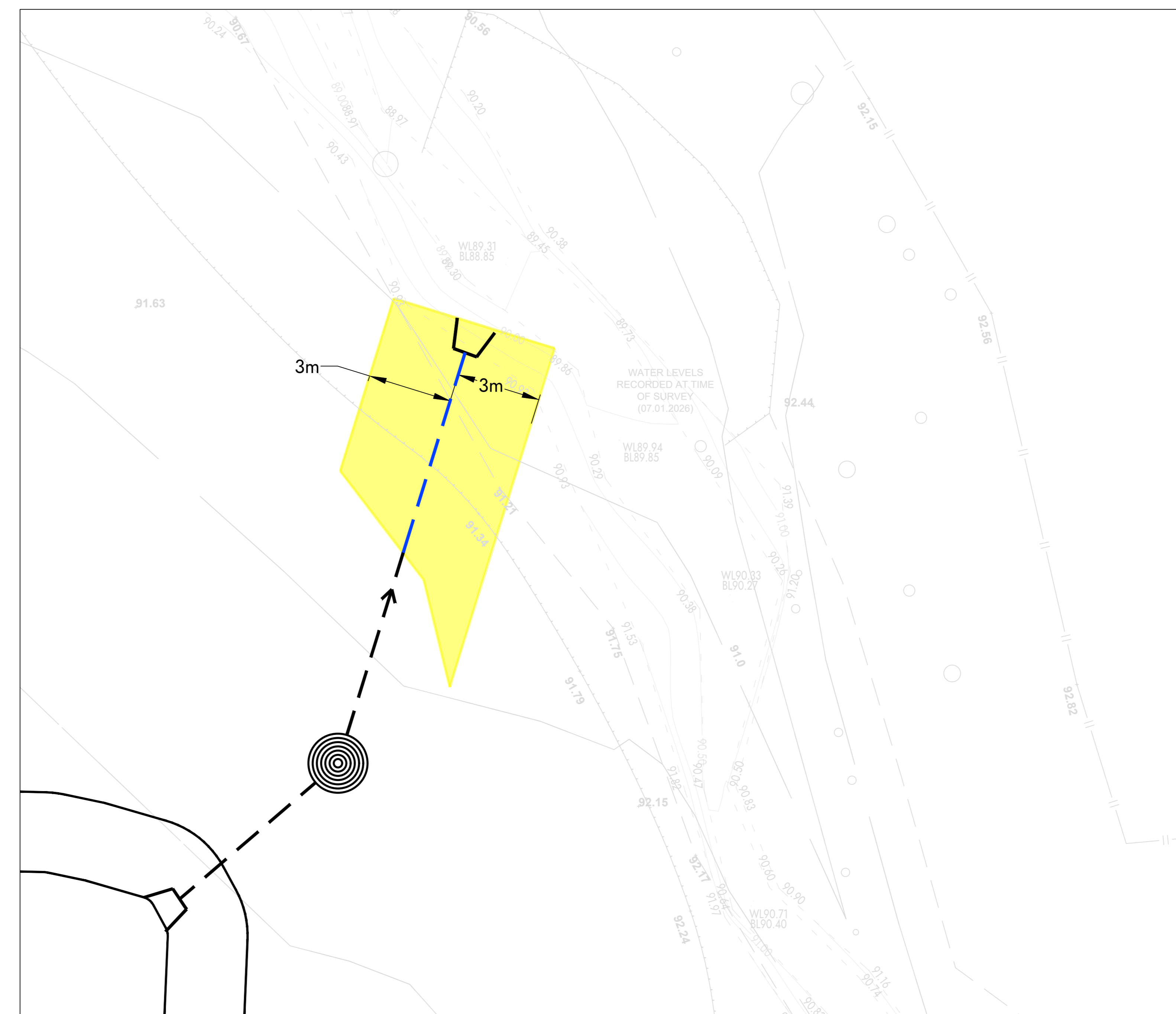
OUTFALL EASEMENT PLAN @ 1:100
