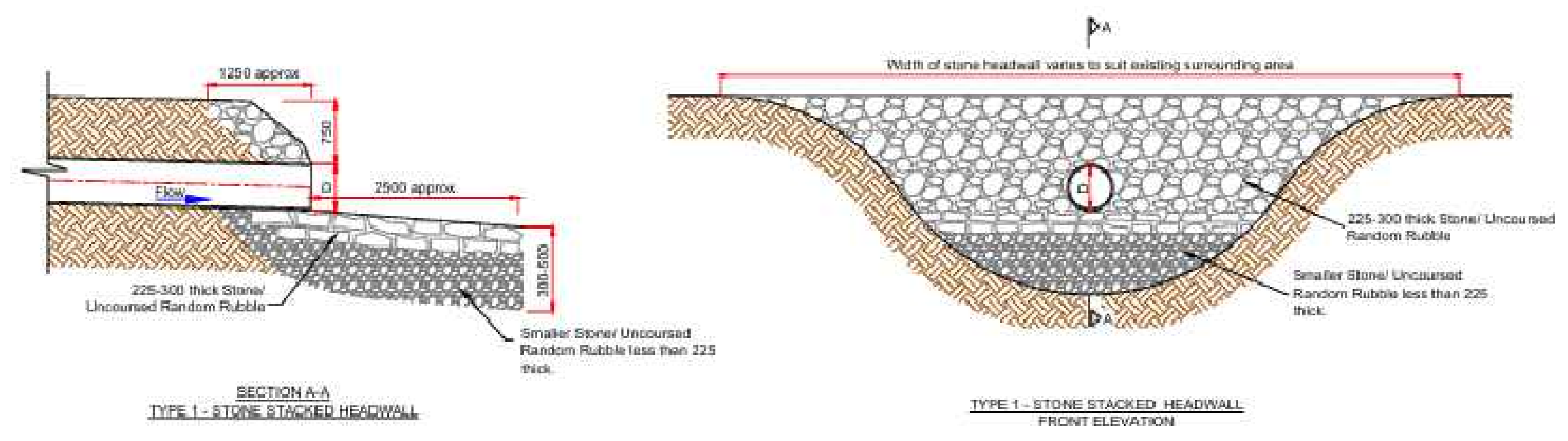
TYPICAL OUTFALL HEADWALL DETAILS (UU TYPICAL TYPE 1 HEADWALL DETAIL)
