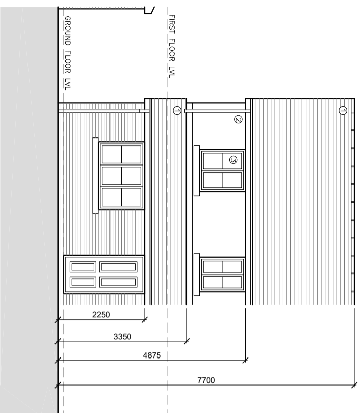
PROPOSED NORTH WEST ELEVATION 1
