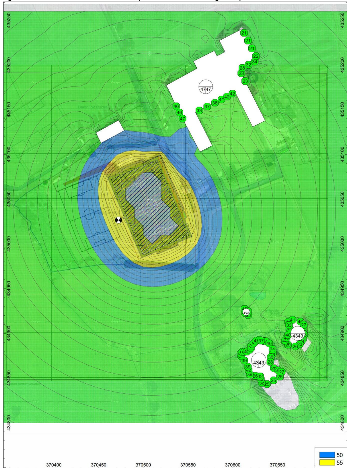
Figure 6: Predicted AGP Noise Emission (4.5 metres above the ground).
