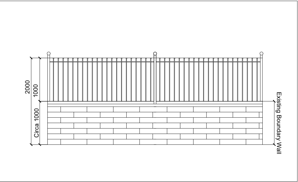
Proposed Fence Elevation, Scale : 1:50
