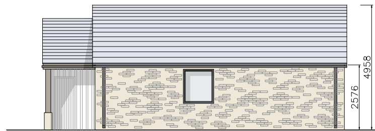
North Elevation
