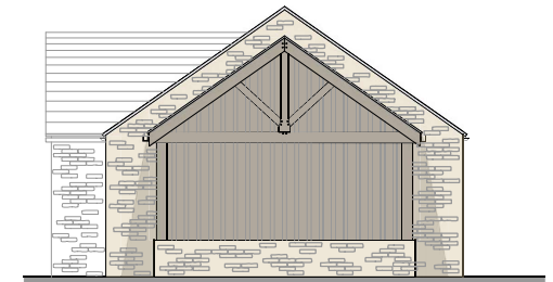
East Elevation
