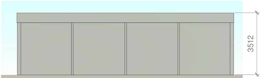
3 East Elevation 1 : 125
