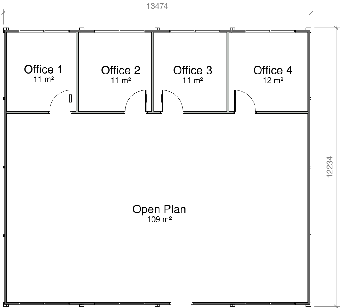
1 Proposed Layout 1 : 100
