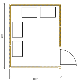
2 proposed plan Scale: 1:50
