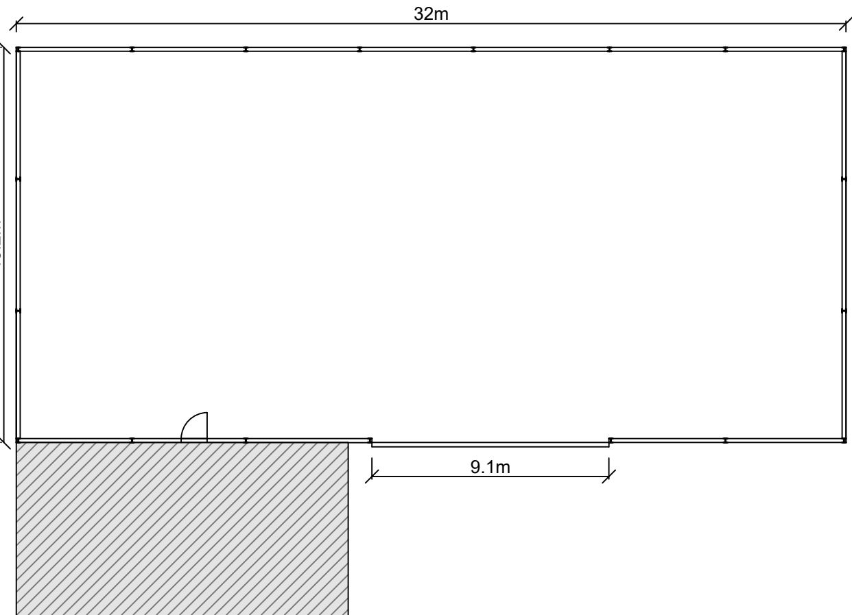
Floor Plan
