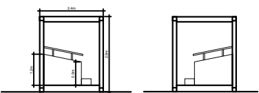
PROPOSED SPECTATOR STAND - SIDE ELEVATIONS SCALE 1:200
