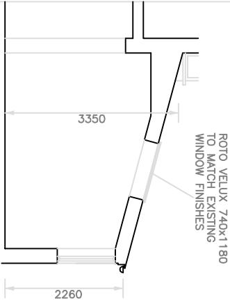
PART SECTION
