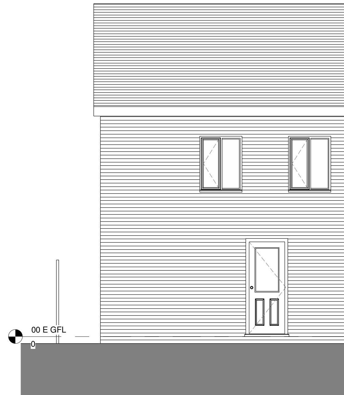
Existing Rear Elevation (part) 1 : 50
