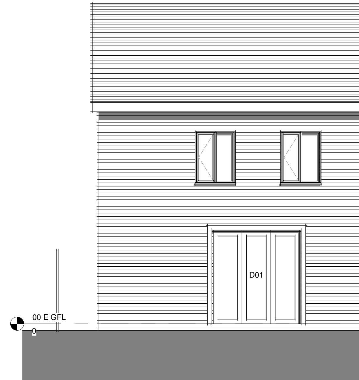
Proposed Rear Elevation (part) 1 : 50
