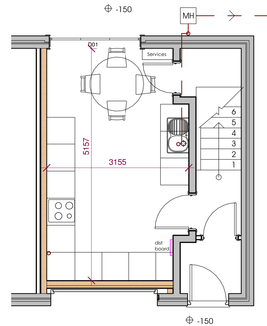
Proposed Ground Floor Plan 1 : 50
