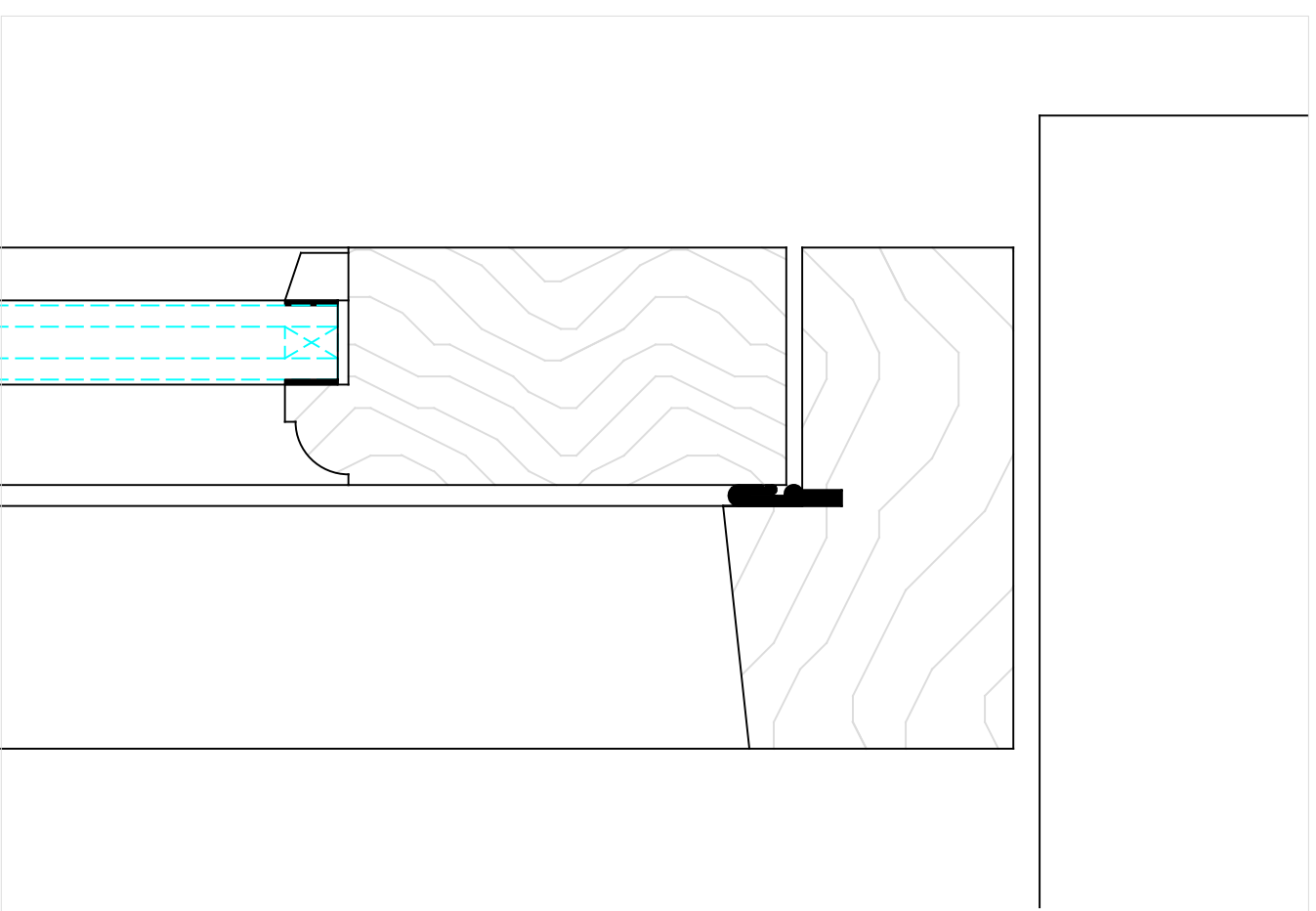
TYPICAL SECTION DETAIL
