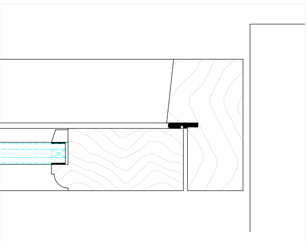
TYPICAL DOOR AND FRAME SECTION SCALE 1-1
