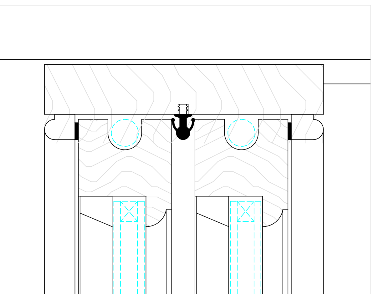
TYPICAL SASH WINDOW DETAIL SCALE 1-1
