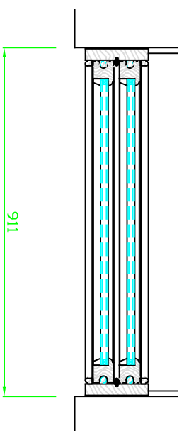
PROPOSED SASH WINDOW PLAN SCALE 1-10
