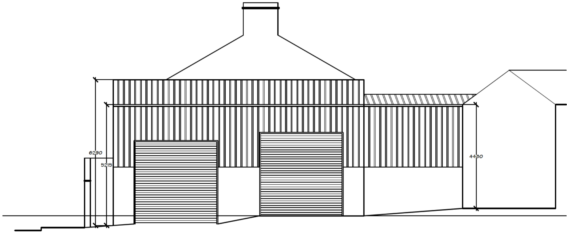
East Elevation
