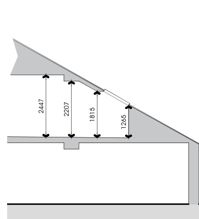
Section
