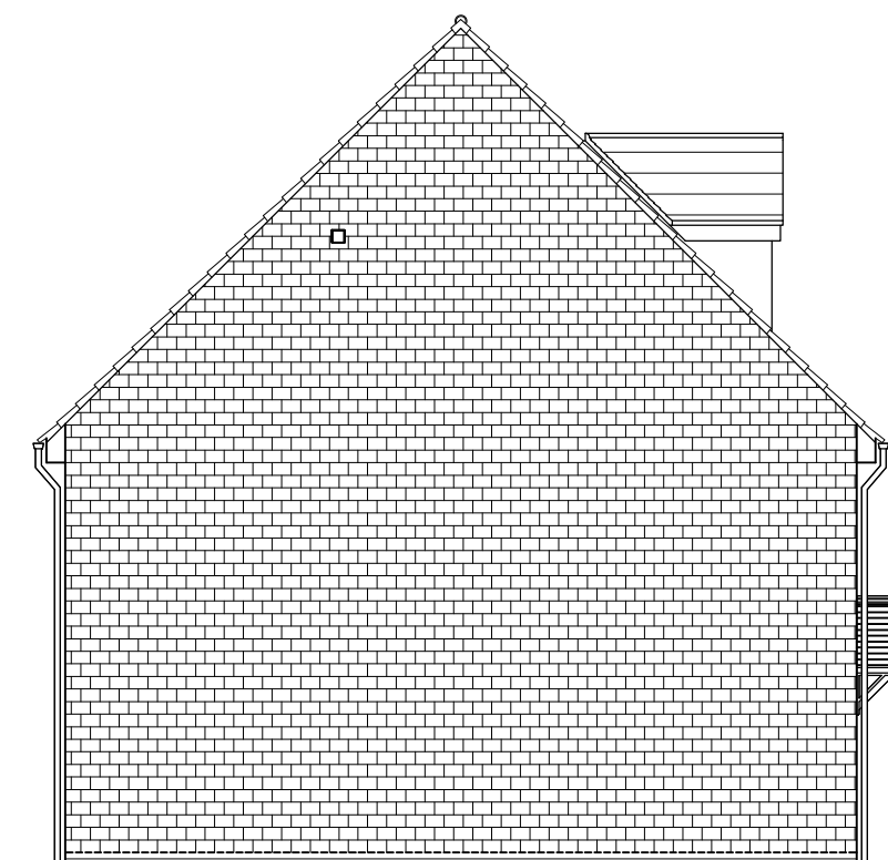
SIDE ELEVATION
