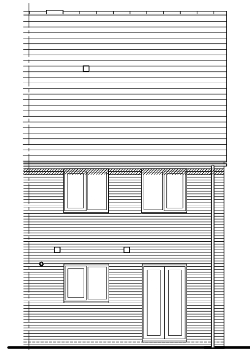
REAR ELEVATION
