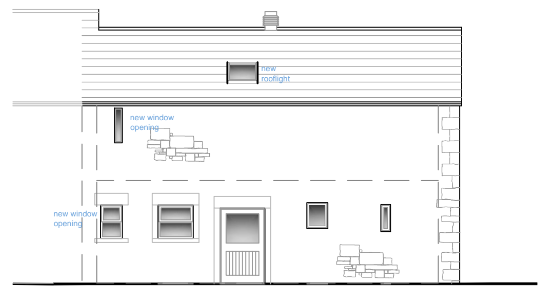
SOUTH ELEVATION
