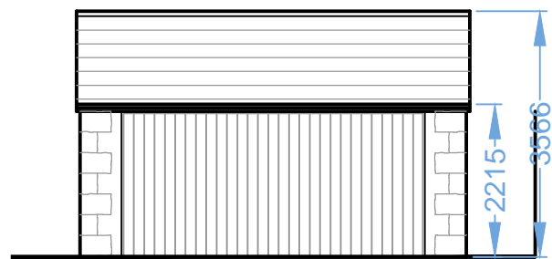
5600 WEST ELEVATION
