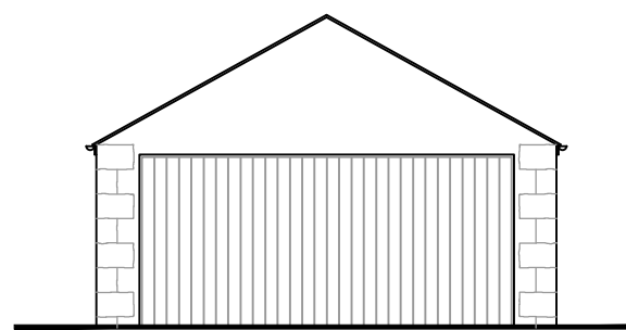
EAST ELEVATION
