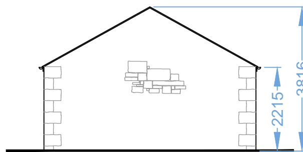
5600 WEST ELEVATION
