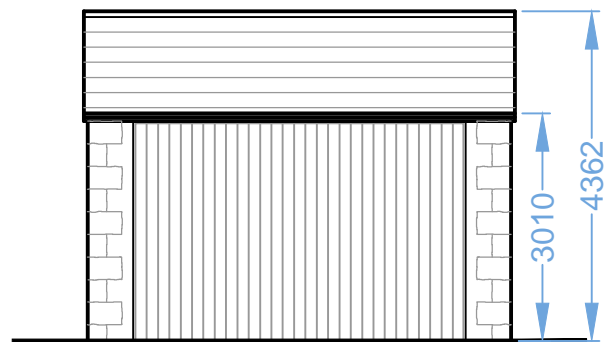
5700 SOUTH ELEVATION
